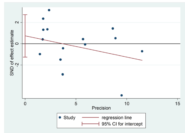
Figure 7. Publication bias.
